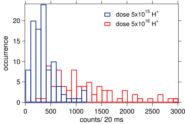
Figure 4: Photoluminescence intensity of smaller than 30 nm PNDs after \text{H}^+ irradiation and annealing : a) Occurrence versus photoluminescence intensity for nanodiamonds irradiated with a dose of 5 \times 10^{15} \text{ H}^+/\text{cm}^2 ; b) Occurrence versus photoluminescence intensity for nanodiamonds irradiated with 5 \times 10^{16} \text{ H}^+/\text{cm}^2 .
