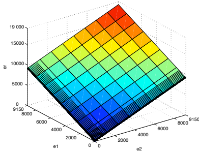
Figure 6: Representation of e_r according to e_1 and e_2 for the approximation of the product c_1 \cdot c_2 for a fixed \alpha . Note that e_r is greater or equal than e_1 and e_2 (the corresponding surface is not a plane).
