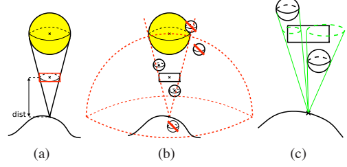
Figure 8: Occluding spheres splatting: (a) a unit square is placed according to the spherical light source; (b) useless blockers are clipped; (c) remaining spheres are splatted onto the unit square.
