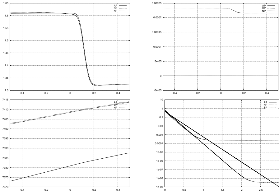
Figure 1: Convergence to a stationary state with a null velocity: \rho , u , p wrt. x for the converged solutions and \|u\|_{L^2} wrt. t (bottom, right)
