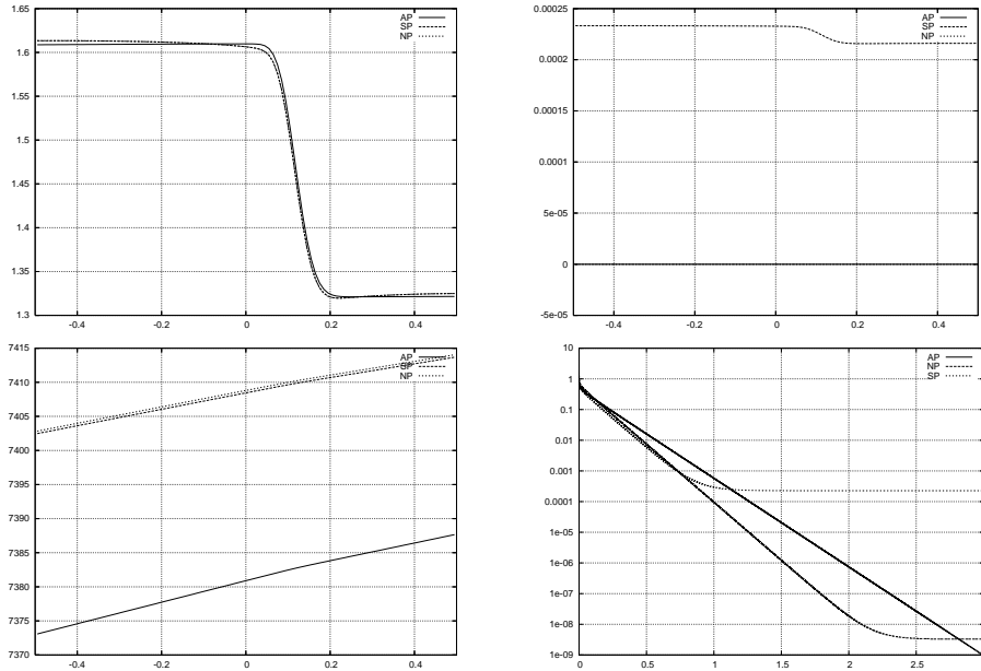
Figure 1: Convergence to a stationary state with a null velocity: \rho , u , p wrt. x for the converged solutions and \|u\|_{\mathbb{L}^2} wrt. t (bottom, right)
