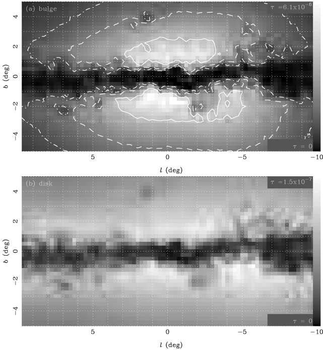
Figure 2. The I -band DIA optical depth maps separately for (a) spheroid+bulge and (b) thin+thick disc lenses. Contours and grey-scales in (a) are as for Fig. 1, whilst the grey-scale range in (b) is 40 times lower than in (a) for clarity of display. The sum of the panels (a) and (b) corresponds to panel (b) in Fig. 1.
