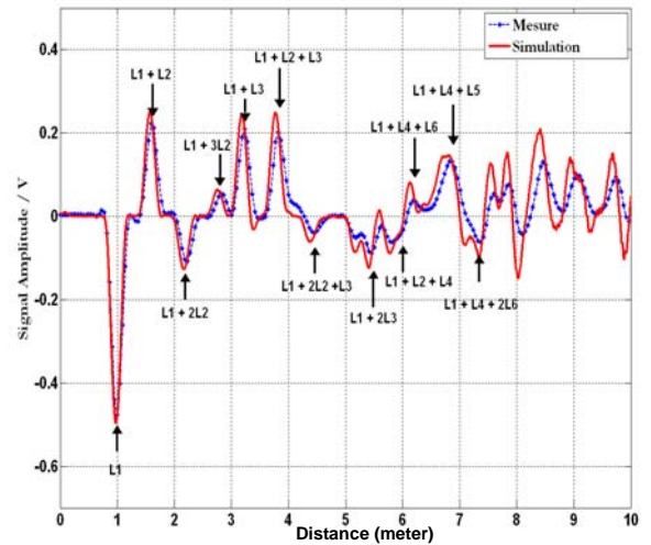
Fig.3. Comparison between simulation results and measures for the TDR response
