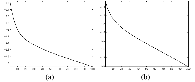
Fig. 4. Decay of the error \log_{10}(\|f^{(l)} - f^*\| / \|f_0\|) for inpainting (a) and deblurring (b).
