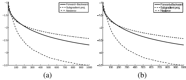
Fig. 2. Decay with k of (a) the error \log_{10}(\|f^{(k)} - f^*\| / \|f^*\|) and (b) of the total variation error \|f^{(k)}\|_{TV} / \tau - 1 for the dual projection (8) (solid line) and the sub-gradient projection [4] (dashed line). Here \tau = \|f_0\|_{TV} / 4 .
