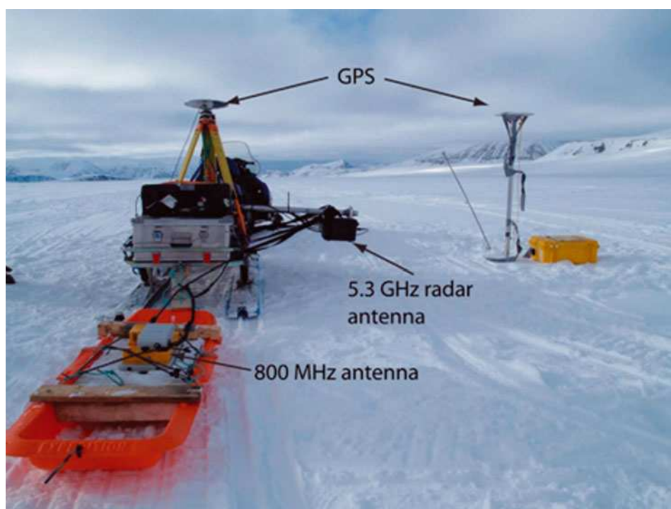
Fig. 2. Field set-up of the radars and GPS. The 5.3 GHz antennas are in the black box protruding to the right of the sledge. The 800 MHz antennas are dragged behind on a plastic sledge.
