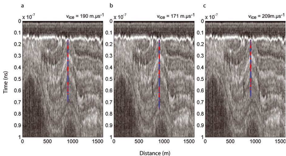
Fig. 6. Comparison of the 5.3 GHz co-polarized radargram with the integrated, normalized, smoothed and thresholded (70%) superimposed ice core. Blue represents low bubble content; red represents high bubble content. Depth-to-time conversion of the core was performed with a velocity of (a) 190 \text{ m } \mu\text{s}^{-1} , the bulk CMP velocity, (b) 171 \text{ m } \mu\text{s}^{-1} and (c) 209 \text{ m } \mu\text{s}^{-1} .
