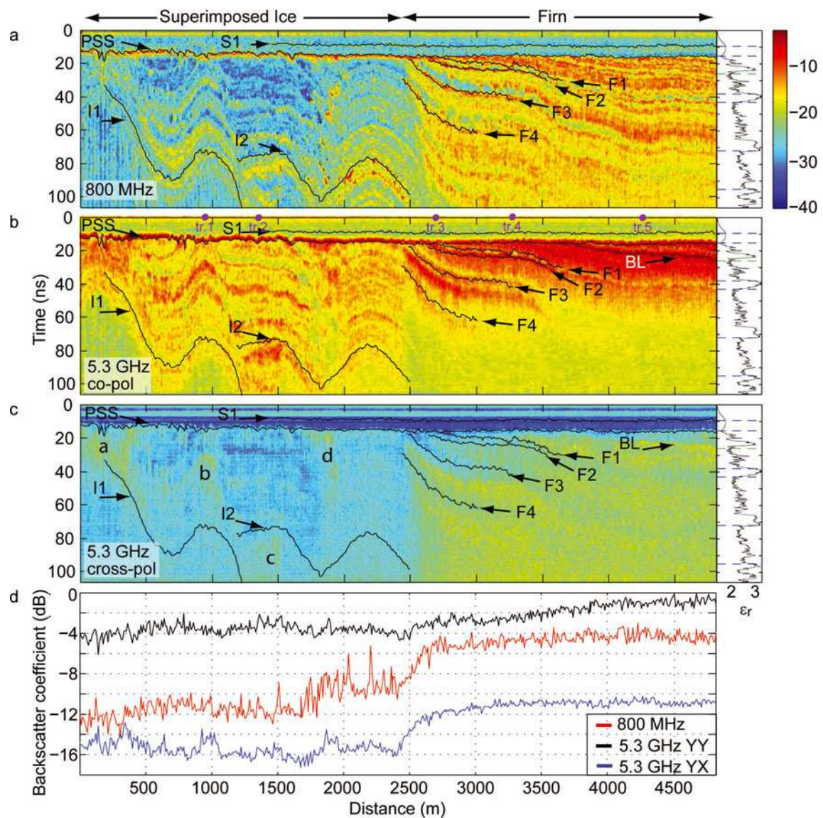
Fig. 5. (a–c) Normalized scattering cross-section, \sigma_{wq} , at (a) 800 MHz, (b) 5.3 GHz YY and (c) 5.3 GHz YX (normalized with respect to YY). Colour bar shows scale in dB. Horizons digitized on the 800 MHz profile in the snow (S1), previous summer surface (PSS), superimposed ice (I1, I2), and firn (F1–F4) are shown as black curves. At the right end of each radargram, a profile of the average permittivity of the five firn cores is shown with the approximate time location of the digitized horizons at stake 8. The points marked tr.1–5 correspond to the locations of the traces in Figure 7. (d) Normalized backscatter coefficient, \sigma_{wq}^0 , along the profile. The 5.3 GHz cross-polarized response is normalized with respect to the co-polarized response, and the 800 MHz profile has been shifted down by 3 dB for ease of comparison.
