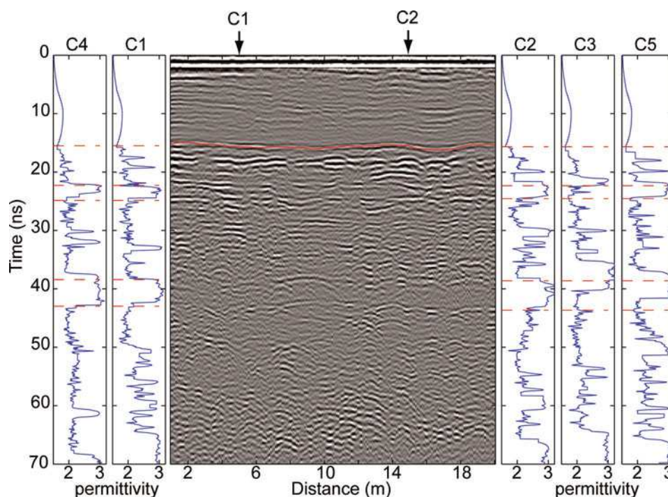
Fig. 8. 800 MHz profile in grid section at stake 8 in the firn area (Fig. 1). The profile passes over cores 1 and 2 at the approximate locations indicated by the arrows. The DEP-derived permittivity profiles for the five cores, C1–C5, are shown either side of the radargram. Red dashed lines show the mean depth (in ns) of the interfaces.
