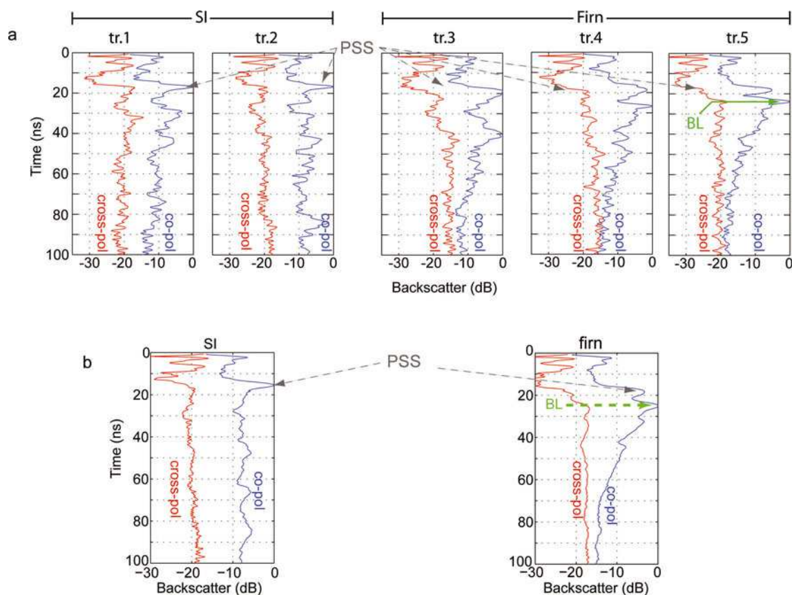
Fig. 7. (a) Traces illustrating the 5.3 GHz co-polarized and cross-polarized normalized scattering cross-section extracted from Figure 5. The cross-polarized response is given in red and the co-polarized response in blue. (b) Co-polarized and cross-polarized backscatter trends over depth for the superimposed ice and firn areas. Each trace is an average of 100 consecutive traces. The PSS response is indicated by the dashed grey arrows. Reflection horizon at the bright layer (BL in Fig. 5 and text) is marked.
