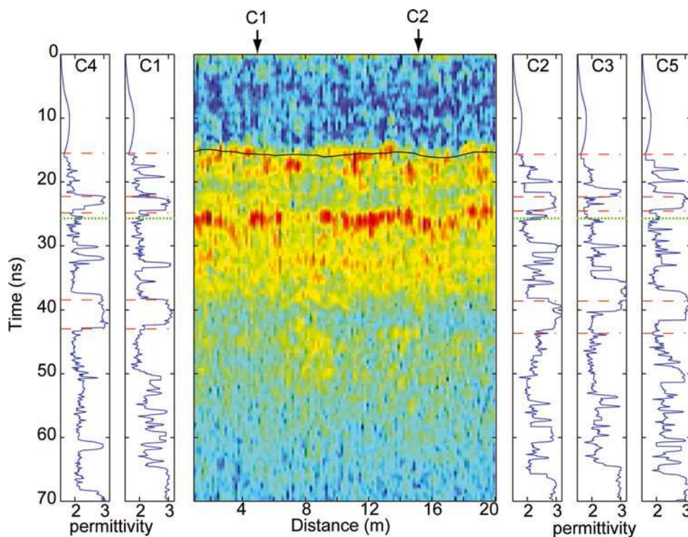
Fig. 9. 5.3 GHz co-polarized profile in the grid at stake 8 in the firn area (Fig. 1). The profile passes over cores C1 and C2. The approximate location of the cores is indicated by the arrows. The DEP-derived permittivity profiles for the five cores, C1–C5, are shown either side of the radargram. Red dashed lines are the mean depth of interfaces digitized on the 800 MHz grid profile. The green dashed line is the mean depth of the bright layer (BL).
