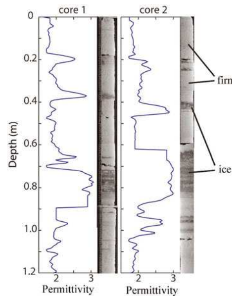
Fig. 4. Digital imagery of the upper sections of firn cores 1 and 2, along with the DEP-derived permittivity profiles. Firn appears white and ice dark. The depth scale starts at the previous year's summer surface.
