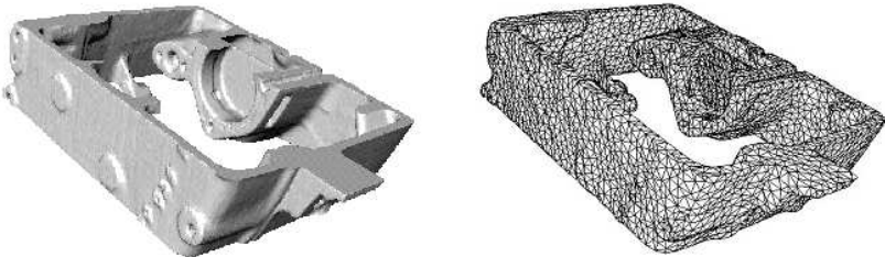
Fig. 1. Scan of a crankcase (courtesy Tomoadour-TurboMéca), generation of a F.E. mesh (total time ~2h), 427132 faces in the initial model and 11924 in the F.E. mesh.
