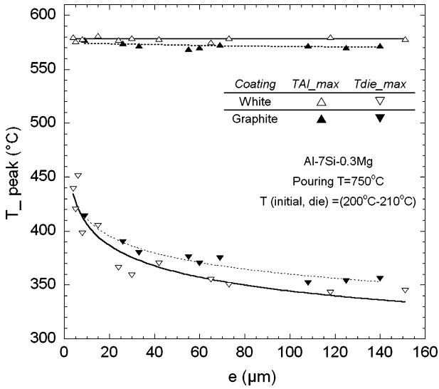
Fig. 7—The variation of die and alloy surface temperature as a function of coating thickness ( e ) for two kinds of coating (white and graphite) during casting cycles of alloy Al-7Si-0.3Mg.
