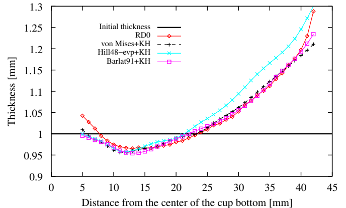
Fig. 23. Comparison between experimental and numerical results for the thickness distributions at the end of forming process in RD for vonMises + KH , Hill48 – evp + KH and Barlat91 + KH criteria with kinematic hardening.
