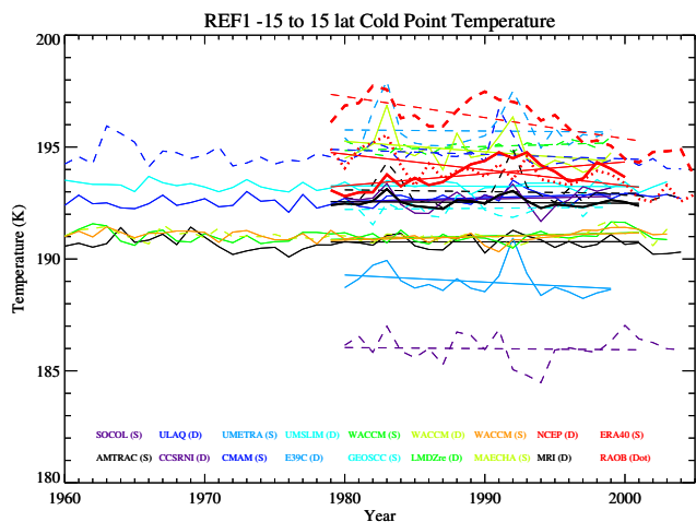
Fig. 4. Tropical mean Cold Point Tropopause Temperature ( T_{CPT} ) from various models for Historical (REF1) runs. Thin lines are linear trends. Models are either solid ( S ) or dashed ( D ) lines as indicated in the legend. Thick red lines are NCEP/NCAR (dashed), ERA40 (solid) Reanalyses and thick red dotted line is radiosonde annual anomalies as described in the text. Thick black line is the multi-model mean anomalies added to the ERA40 inter-annual mean as described in the text.
