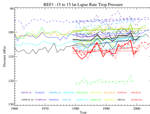
Fig. 5. Tropical mean Lapse Rate Tropopause Pressure ( P_{LRT} ) from various models for Historical (REF1) runs. Thin lines are linear trends. Models are either solid ( S ) or dashed ( D ) lines as indicated in the legend. Thick red lines are NCEP/NCAR (dashed), ERA40 (solid) Reanalyses and thick red dotted line is radiosonde annual anomalies as described in the text. Thick black line is the multi-model mean anomalies added to the ERA40 inter-annual mean as described in the text.
