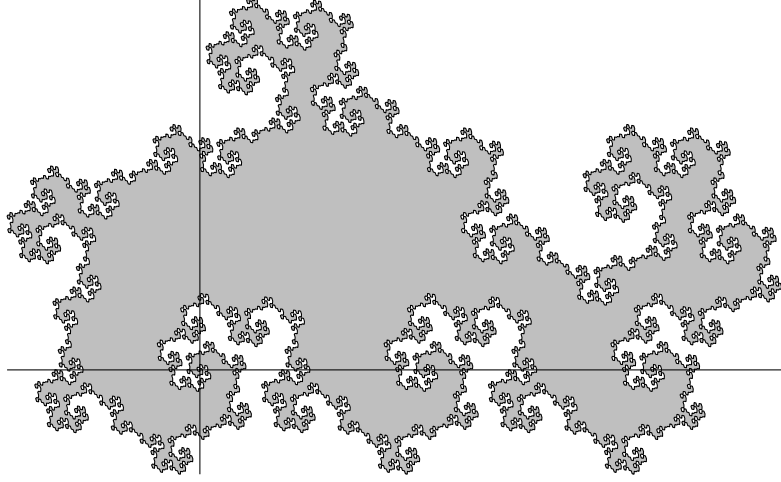
FIGURE 5. The central tile associated with the real root of x^3 - 3x^2 + 2x - 1 .
