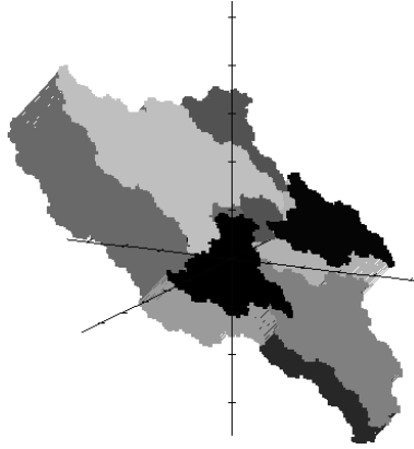
FIGURE 4. The set \mathcal{E}_\eta .
