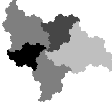
FIGURE 3. The decomposition of the central tile associated with \eta into subtiles. According to the expansion d_\eta(1) = 10001 , the central tile is subdivided into exactly five subtiles.
