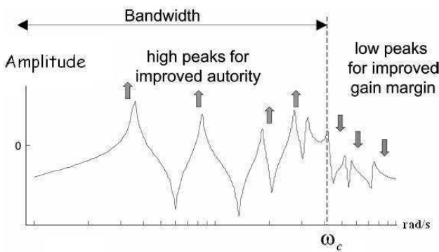
Fig. 3. Desired form of the open-loop FRF.
