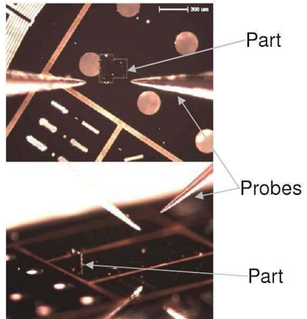
Fig. 1. NIST Part Before and After Insertion
