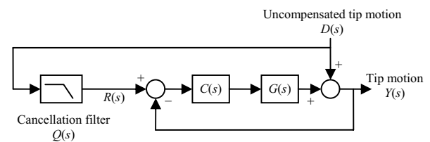
Fig. 3. Small-signal model including cancellation filter.
