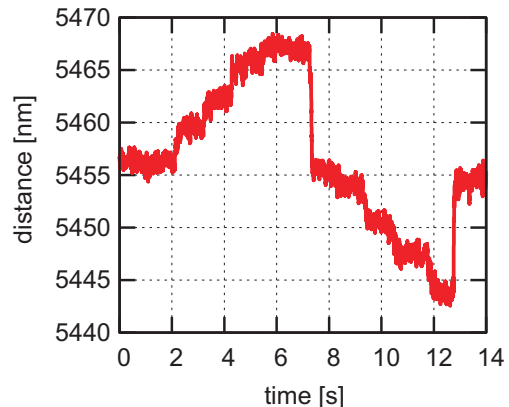
Fig. 4. Force measurements when pushing a CNT against a gripper jaw.
