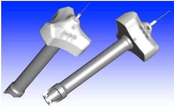
Fig. 1. Two views of the exterior housing of Micron, showing the handgrip and the three-pointed star-shaped manipulator, with the four LEDs that are used for optical tracking.
