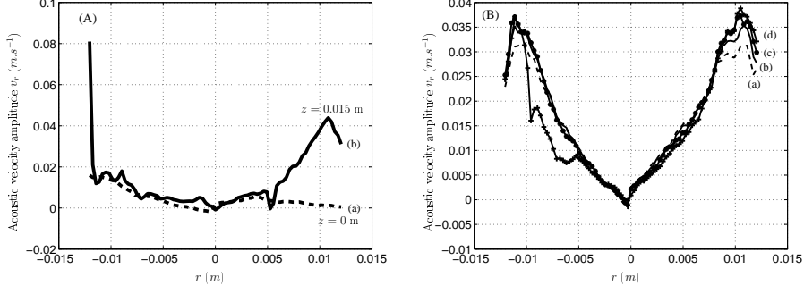
Fig. 6. (A) Radial acoustic velocity amplitude v_r as a function of r for z = 0 m (a) and z = 0.015 (b). (B) Radial acoustic velocity amplitude v_r as a function of r for (a) z = 0.0136 m ( \dots ), (b) z = 0.0139 m ( --- ), (c) z = 0.0142 m ( * ) and (d) z = 0.0145 ( + )
