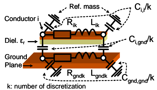
Figure 2: Parasitic capacitance location
