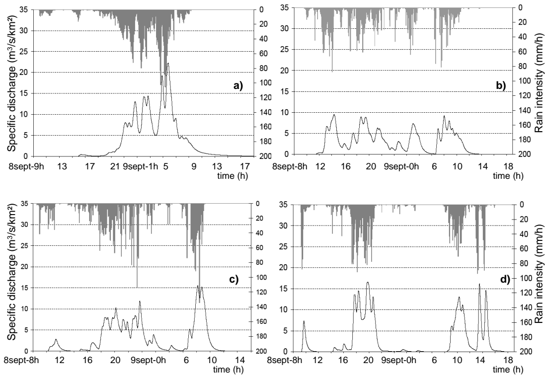
Fig. 8. Simulated discharges at the (a) Rousson ( 12 \text{ km}^2 ), (b) Saint Quentin la Poterie ( 12 \text{ km}^2 ), (c) Quissac ( 2 \text{ km}^2 ) and (d) Domazan ( 6 \text{ km}^2 ) outlets. See Fig. 1 for the locations.
