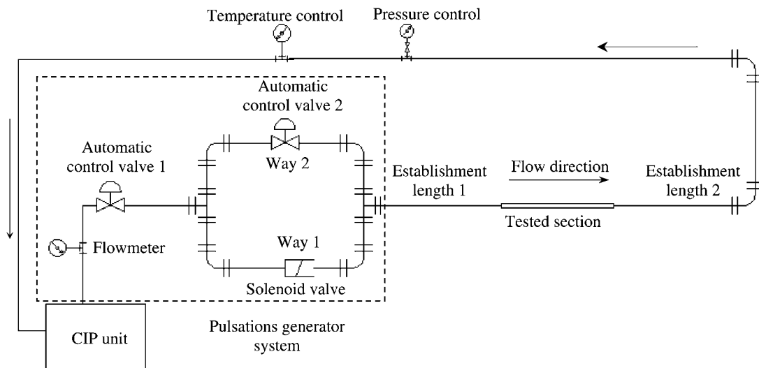
Fig. 1. Schematic diagram of the pulsation generation system and the tested section.
