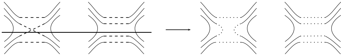
FIG. 9: Covariances C_\sigma (dashed lines) sandwiched in the inner product in the Cauchy-Schwarz inequality (thick line) are replaced by modified covariances C'_\sigma (dotted lines).
