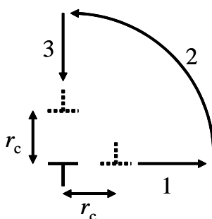
Figure 2. Reversible thermodynamic cycle for a dipole of edge dislocations.
