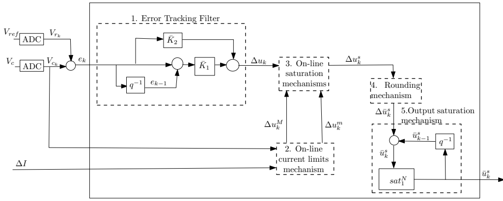
Fig. 5. ENARC structure patented in [10].
