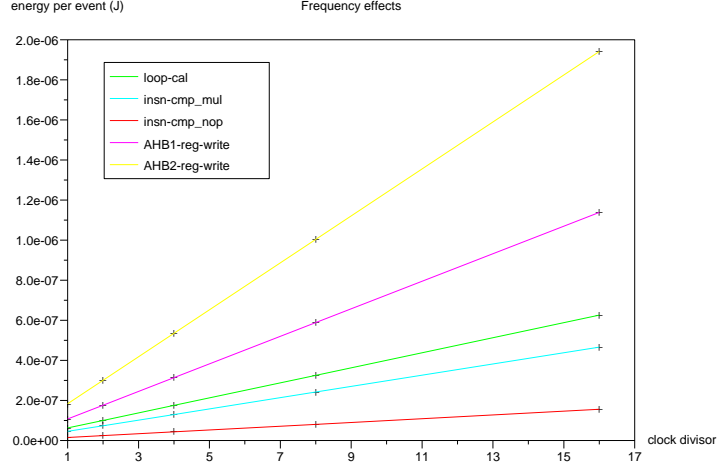
Figure 9: Multiple frequencies experiments : This figure shows that the energy per event increases linearly against frequency ratio.
