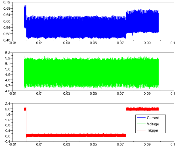
Figure 6: Acquisition results : the two upper graphs are interesting data i and v , and the lower one is the trigger signal LED
