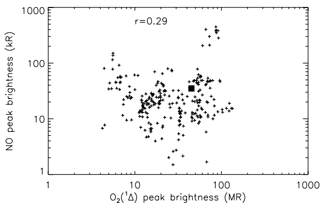
Figure 6. Brightness distribution of the emission peaks of the NO and O 2 ( 1 Δ) airglow layers measured quasi-simultaneously at the limb. The observations corresponding to each point have been determined as illustrated in Figures 3 and 4 (see text). The correlation coefficient is 0.29 , indicating the lack of covariation of the brightness of the two emissions. The full square indicates the mean value of the peak intensity of the two emissions.
