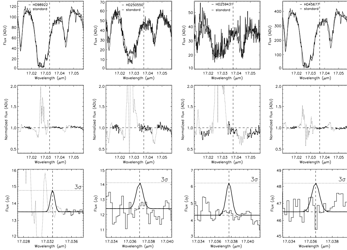
Fig. 1. Spectra obtained for the H 2 S(1) line at 17.0348 \mu\text{m} . Top panel: continuum spectra of the standard star and of the target before telluric correction. Central panel: full corrected spectra: dotted lines show spectral regions strongly affected by telluric features. Bottom panel: zoom of the region where the S(1) line should be observed (dashed vertical lines). A Gaussian of width FWHM = 21 \text{ km s}^{-1} and integrated line flux equal to the 3\sigma line-flux upper limits is overlotted. The spectra were corrected neither for the radial velocity of the targets nor the Earth’s rotation velocity.
