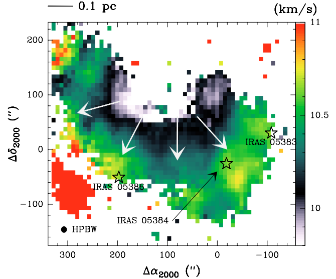
Fig. 3. Map of the C^{18}O(2-1) velocity centroids. Indicated by stars are three IRAS sources identified by Sandell et al. (1986). The arrows indicate the velocity gradient orientations at different positions across the neck and ridge.
