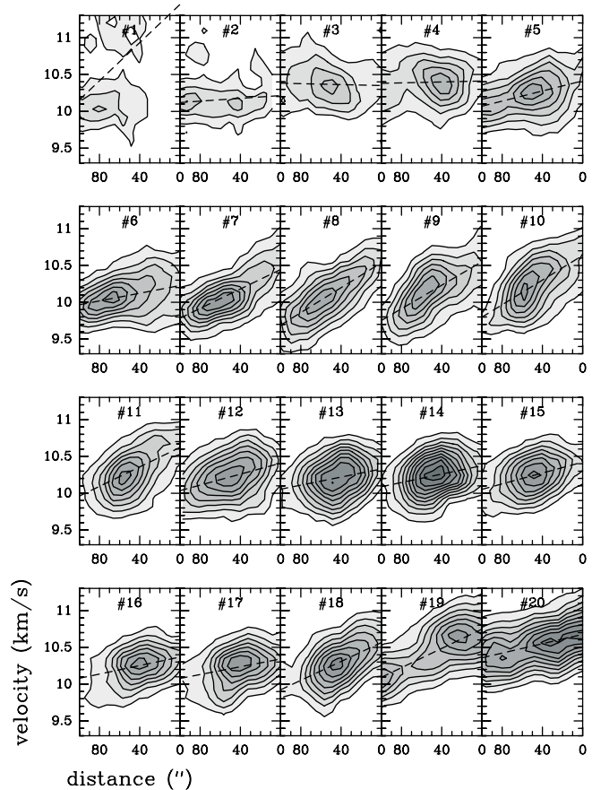
Fig. 8. Transverse \text{C}^{18}\text{O}(2-1) position-velocity cuts performed across the neck, corresponding to the black thin lines of Fig. 5. The cuts are separated by 22'' . The x -axis offsets increase northwise, so that the velocity decreases from South to North. Dashed lines indicate the results of the bi-dimensional fits to the l-v diagram (see text for details), showing how the radial velocity gradient evolves as one moves from East to West (cf. Fig. 9). Contours start at 3\sigma ( 0.6 \text{ K} ), in steps of 3\sigma .
