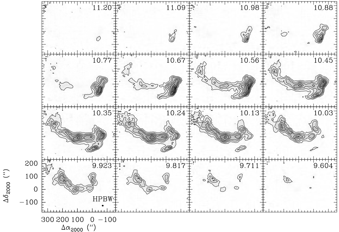
Fig. 2. Channel maps of the \text{C}^{18}\text{O}(2-1) emission between 9.6 and 11.2 \text{km s}^{-1} . Contours are 1.1 K to 7.4 K by steps of 0.9 K ( T_{\text{A}^*} scale, rms = 0.2 K).
