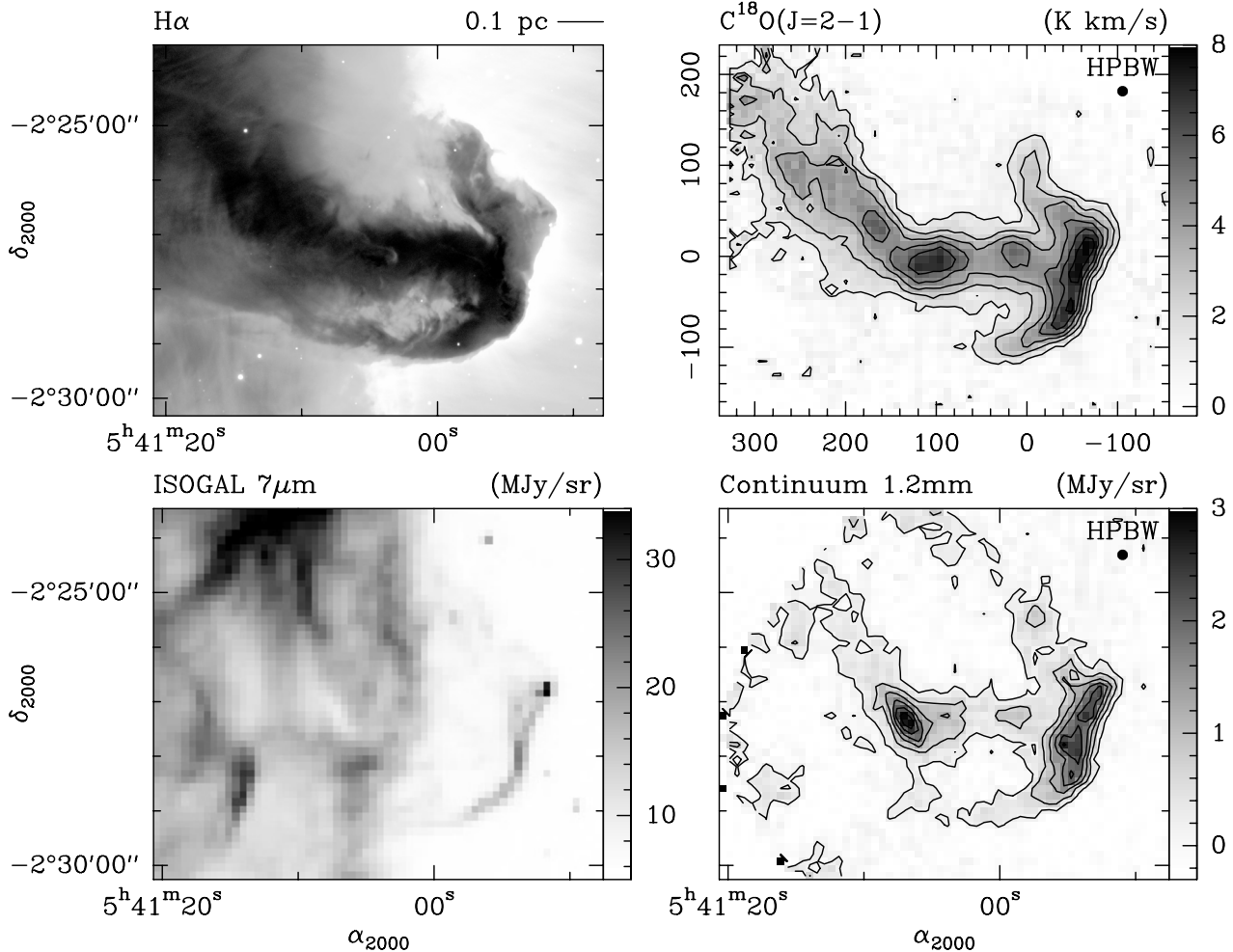
Fig. 1. Upper left: H\alpha line emission map obtained at the 0.9 m KPNO telescope (courtesy of Reipurth & Bally). Upper right: integrated emission map ( \int T_{mb,c} dv , K \text{ km s}^{-1} , v \in [9.1:11.8] \text{ km s}^{-1} ) of C^{18}O(2-1) . Offsets are in arcsec and contours are 1.2 to 7.2 by 1.2 K \text{ km s}^{-1} . The half-power beam width (HPBW) is plotted at the top right corner. Bottom left: continuum emission around 7 \mu\text{m} (mostly aromatic emission) covered by ISO. Bottom right: continuum emission at 1.2 mm observed by MAMBO2. Contours are 0.15 MJy/sr to 2.65 MJy/sr by 0.5 MJy/sr.
