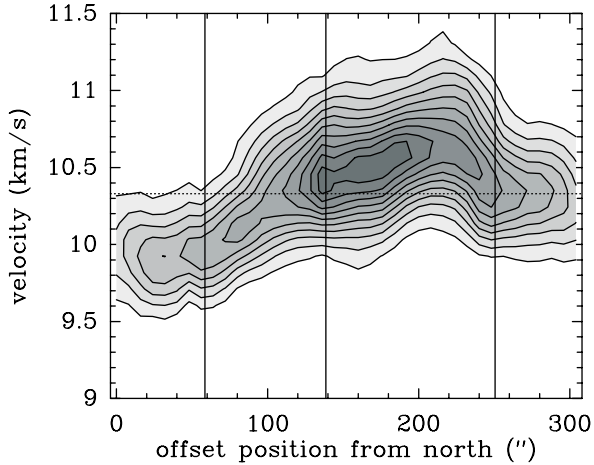
Fig. 6. \text{C}^{18}\text{O}(2-1) position-velocity cut performed along the western ridge and the mane (from north to south, Fig. 5). The dashed horizontal line indicates the systemic velocity v_0 . The three vertical lines delineate the four segments forming the cut. A large ( +2.6 \text{ km s}^{-1} \text{ pc}^{-1} ) north-south velocity gradient is observed until the mane, where the gradient is suddenly inverted to finally end up at the systemic velocity with a slope of -4.3 \text{ km s}^{-1} \text{ pc}^{-1} . Contours start at 3\sigma ( 0.6 \text{ K} ), in steps of 3\sigma .
