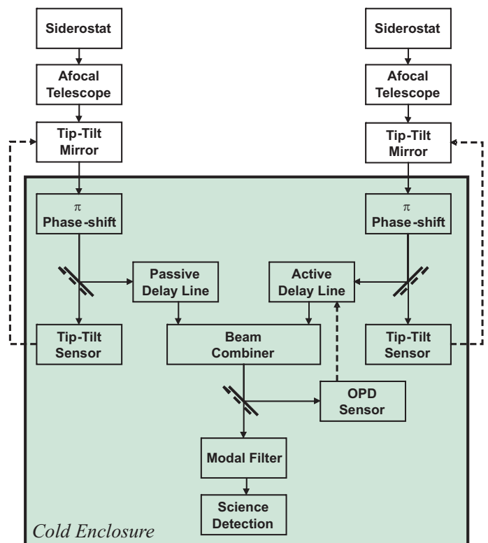
Fig. 2. Block diagram of the ALADDIN optical architecture. Feed-back signals driving the control of the tip-tilt and OPD parameters are shown in dashed lines. The entrance windows of the cold enclosure are not represented, for simplicity.
