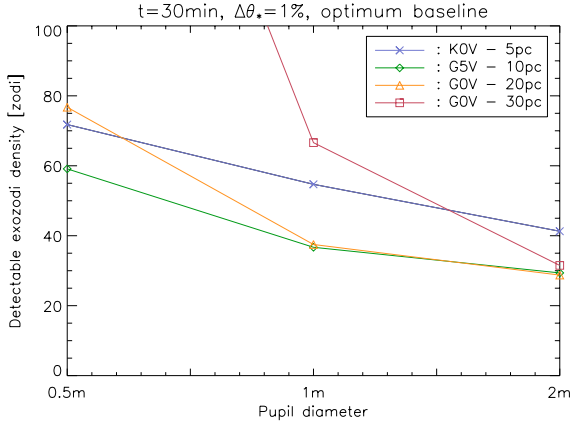
Fig. 7. Simulated performance of ALADDIN in terms of exozodiacal disc detection for three different pupil diameters (50 cm, 1 m and 2 m).
