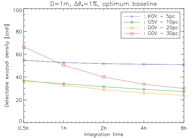
Fig. 6. Simulated performance of ALADDIN in terms of exozodiacal disc detection for increasing integration times.
