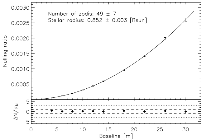
Fig. 5. Simultaneous fit of the stellar radius and the exozodiacal density level using ten 30-min observations of a K0V star at 5 pc (actual radius of 0.85 R_{\odot} ), surrounded by a 50-zodi disc. The nulling ratio is computed as the ratio between the destructive and constructive outputs of the beam combiner. The contribution of instrumental stellar leakage to the nulling ratio has been subtracted from this data using the same procedure than elaborated for GENIE: the observation of a calibration target of similar type and distance, but without circumstellar material.
