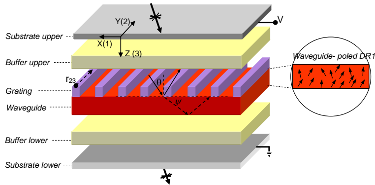
Fig. 1. Active polymer-based grating waveguide structure with an E-O polymer waveguide.
