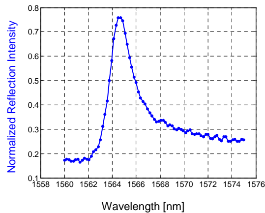
Fig. 3. Experimental normalized reflection intensity as a function of wavelength, for a polymer-based GWS.
