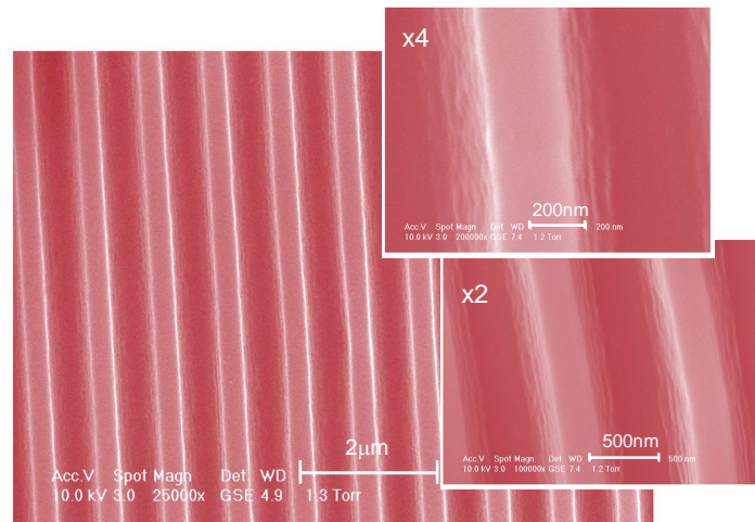
Fig. 2. SEM images of the grating layer. Inserts showing enhanced images of the grating surface roughness.
