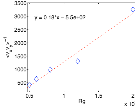
Fig. 8. Mean transport as a function of critical Reynolds number on the anticyclonic side (normalized by S^2 d^2 ).
