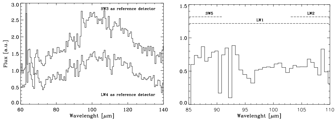
Fig. 4. The 90–110 \mu\text{m} excess in L1551-IRS5, derived using two different reference detectors ( left panel ): SW3 (upper curve) and LW4 (lower curve), as described in the text and shown in Fig. 1. The right panel presents the ratio of these two spectra as well as the range of the SW5, LW1 and LW2 detectors.
