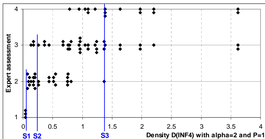
Figure 7. Experts' opinions versus condition grade (84 experts' judgments on 30 links). Thresholds S1, S2 and S3 (obtained for CFN / CFP = 2 and for the favorable procedure) are represented on the figure: S1 = 0.064, S2 = 0.251 and S3 = 1.371.
