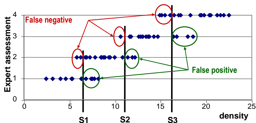
Figure 4. Ideal experts' opinion versus condition grades obtained by comparing scores with thresholds (63 fictitious sewer segments): identification of assignment errors.
