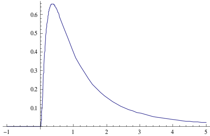
Figure 2: Log-Normal distribution
