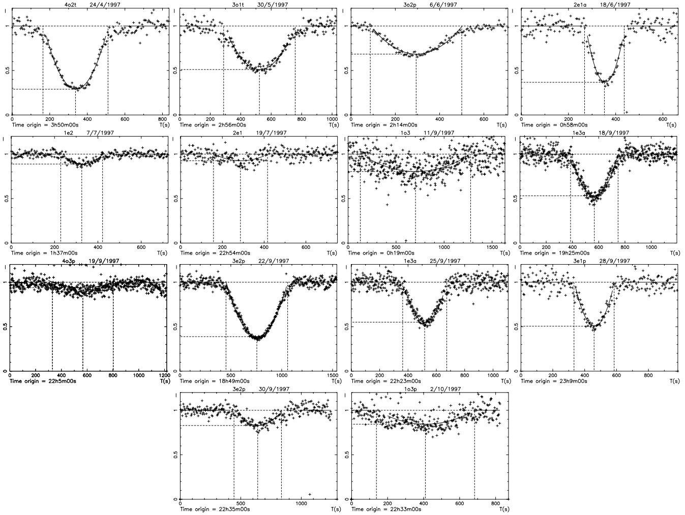
Fig. 1. Light curves of the 14 detected mutual events observed at the Bordeaux Observatory during the PHEMU97 campaign. The intensity I of the eclipsed or occulted satellite is linearly fitted out of event and polynomially fitted during event. The flat level of satellite intensity out of event is normalized to the arbitrary value I = 1 . Time argument T is expressed in seconds of Universal Time (UT).
