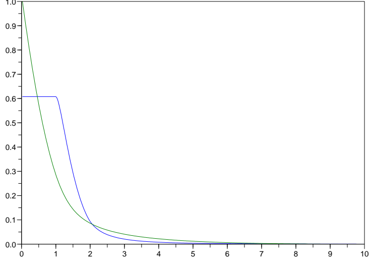
FIGURE 1. The graphs of \Upsilon (green curve) and of p (blue curve)
