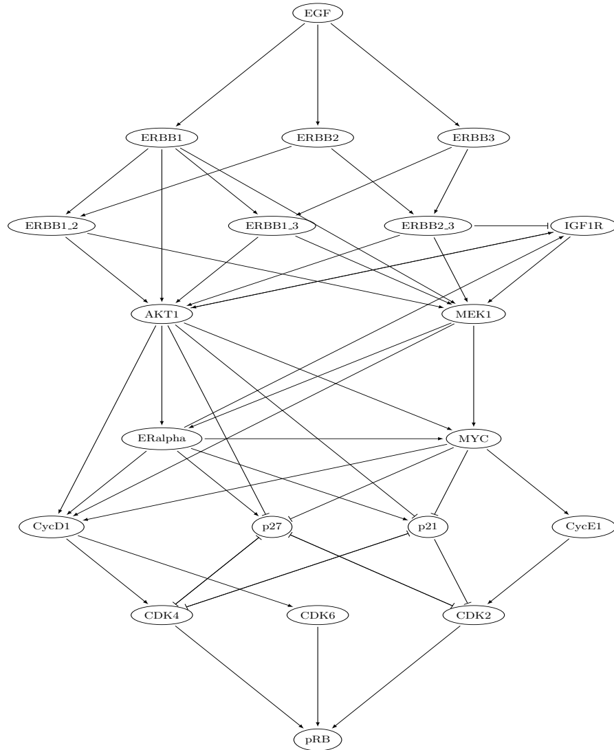
Fig. 7. ERBB receptor-regulated G1/S transition GRN reproduced from
