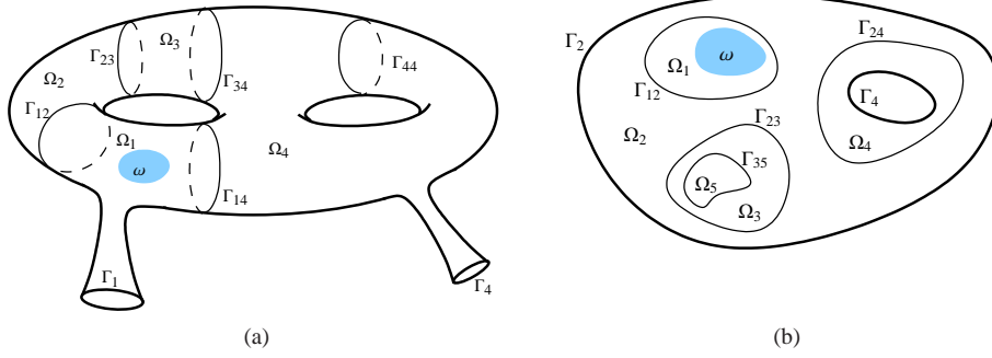
Figure 2: (a) General geometrical configuration: M is a compact manifold with boundary. (b) A particular case: M is an bounded open subset of \mathbb{R}^n .
