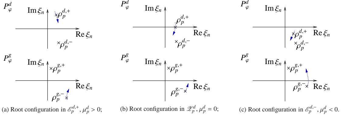
Figure 1: The root \rho_p^{d,+} crosses the real axis before the root \rho_p^{g,-} does, as \mu_p^d decreases.
