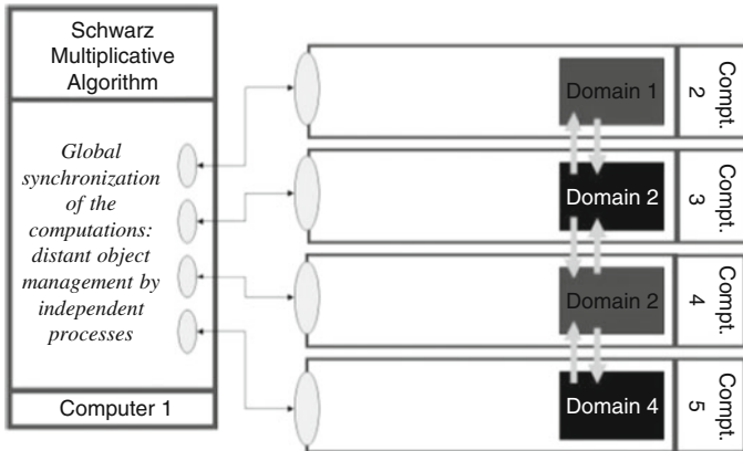
Distributed application
