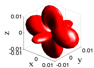
FIG. 1: (Color online) Angular distributions of the C-H bonds (left column) and molecular axes (right column) calculated at t = 8.3 ps after the excitation of an ethylene molecule by a pulse of peak intensity I = 20 TW/cm 2 and pulse duration \tau_{\text{FWHM}} = 100 fs. The temperature is T = 0.1 K. (a) Linearly polarized laser pulse ( a^2 = 0 ). (b) Elliptically polarized laser pulse with a^2 = 0.44 . The structure of C 2 H 4 and the body-fixed frame is shown in the inset.
