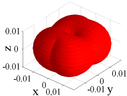
FIG. 7: (Color online) Angular distribution of the C–H bonds of ethylene calculated at t = 8.3 ps for an ellipticity a^2 = 0.44 and a temperature T=4 K. The intensity 5 \text{ TW/cm}^2 is chosen as the averaged values of director cosines to be identical to that obtained in the experiment at T=40 K.
