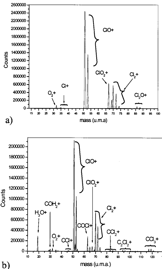
FIG. 5. Mass spectra achieved (a) on a SiO 2 -blanket wafer and (b) on a resist-blanket wafer exposed to the following plasma conditions: Cl 2 (70 sccm)/O 2 (30 sccm)/bias(50 W)/source(500 W)/pressure(10 mT).
