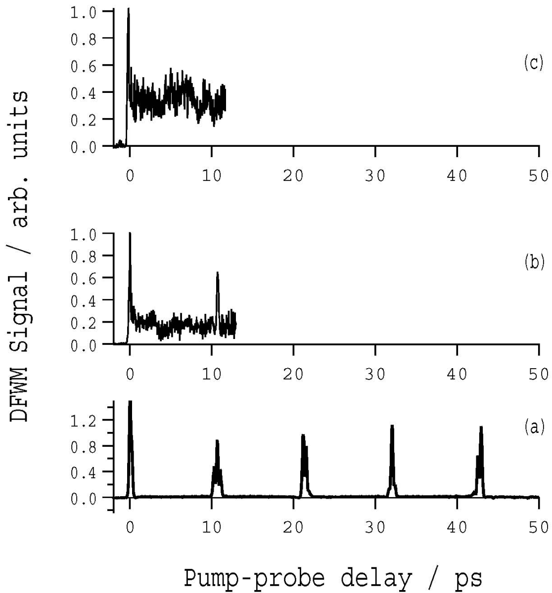
Figure 2 : Evolution of the DFWM signal recorded with parallel pump polarizations at room temperature and at 100 mbar pressure. The intensity for each pump is 18 (a), 36 (b), and 70 TW/cm 2 (c).
