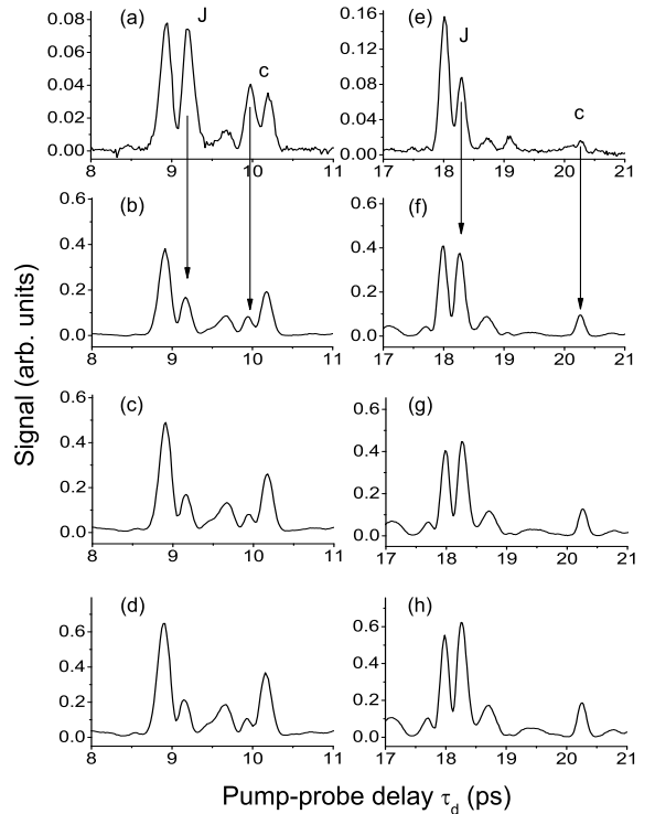
FIG. 6: Probe signals recorded in ethylene exposed to different intensities of the alignment laser: (a, e) 2 \times 10^{12} W.cm ^{-2} , (b, f) 16 \times 10^{12} W.cm ^{-2} , (c, g) 30 \times 10^{12} W.cm ^{-2} , (d, h) 50 \times 10^{12} W.cm ^{-2} . Only the temporal windows that correspond to the first (a-d) and second (e-h) rotational revivals of Fig. 5 are shown.
