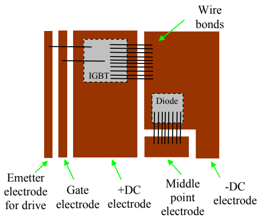
Figure 14: Planar module layout used for measures and simulation.
