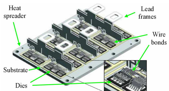
Figure 1: 3D view of a planar power module 3.3 kV, 1200 A [5]
