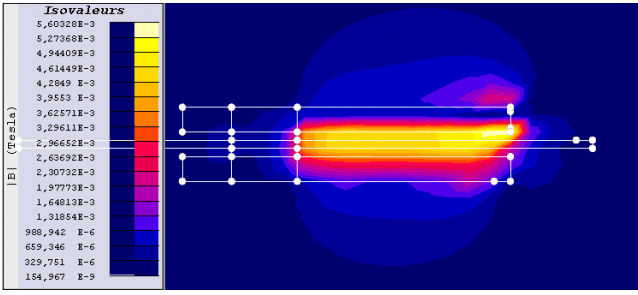
Figure 18: Induction of a Chip on Chip buck converter (side view).
