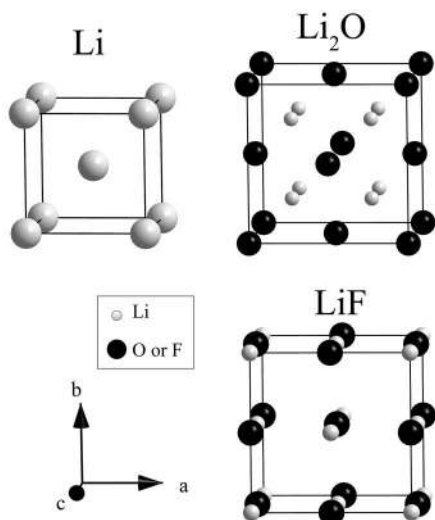
FIG. 1. Unit cells of Li, \text{Li}_2\text{O} , and LiF. These crystal structures can respectively be described in the following space groups: Im\bar{3}m , Fm\bar{3}m , and Fm\bar{3}m .
