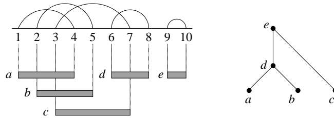
Fig. 1: An involution in \mathcal{I}_{10} , the corresponding collection of intervals and the associated (\mathbf{2} + \mathbf{2}) -free poset.
