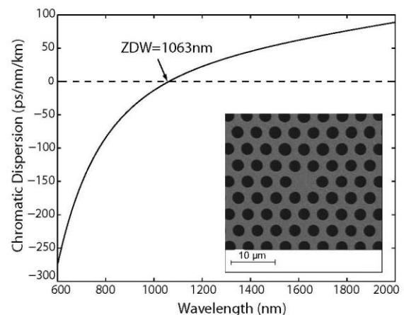
FIG. 1. Chromatic dispersion vs wavelength. Inset: SEM image of the solid-core PCF.
