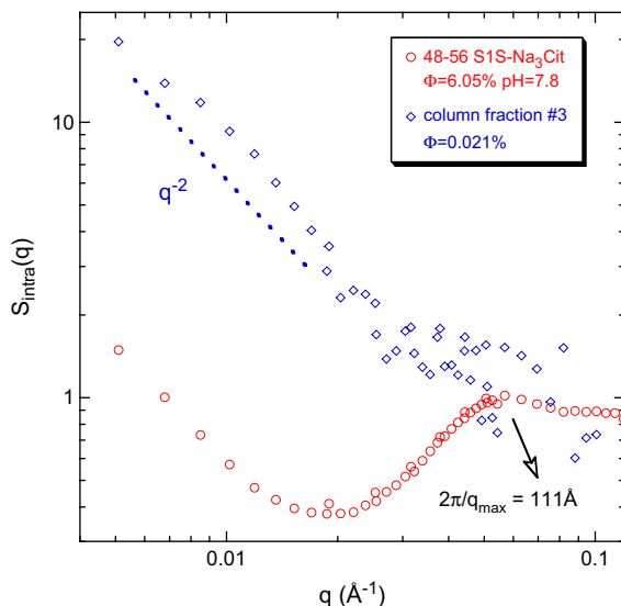
Fig. 5. SANS curves for PB_{48}\text{-}b\text{-}PGA_{56} vesicles prepared in the citrated ferrofluid S1S- \text{Na}_3\text{Cit} before and after column fractionation.
