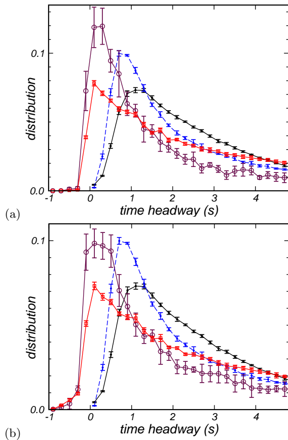
FIG. 6: (Color online) On both figures: intra right and left lane time headway distributions (resp. solid black and dashed grey — blue online — lines). Fig.(a): distributions of the time headway with the left-lane predecessor, for (maroon online — circles) the inter-lane procedure of fig. 5a, or for (red online — squares) the random procedure of fig. 5c. Fig.(b): same as fig. (a), but it is now the successor that is considered on the left-lane. The random procedure (red online — squares) corresponds now to the procedure of fig. 5e.
