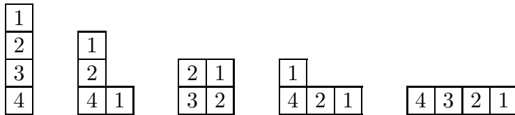
Fig. 2. partitions of 4 and the hook lengths h_v
