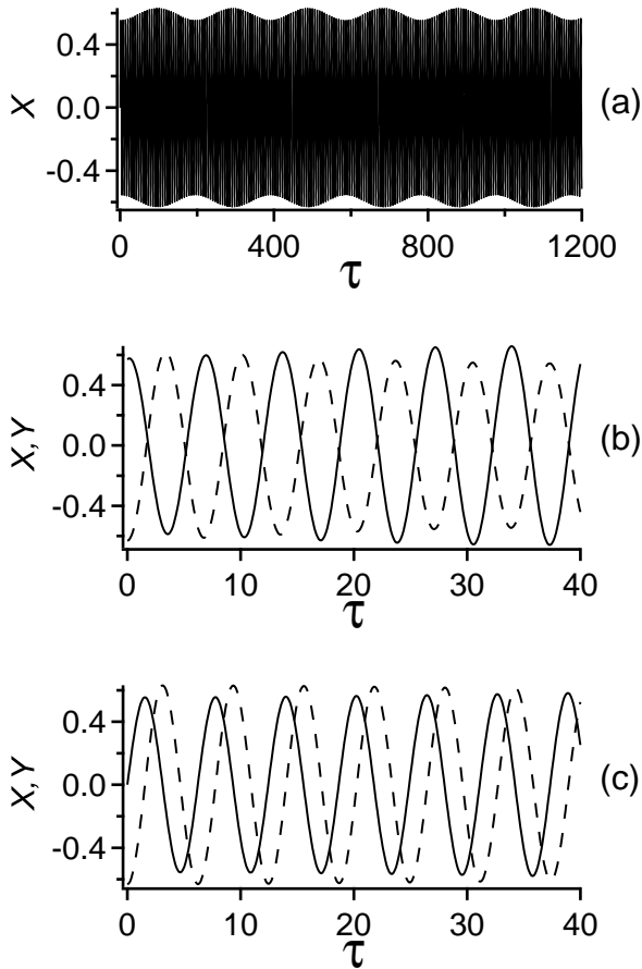
Figure 3: Motion of the atoms as a function of the time \tau = \omega_0 t , for \alpha = 0.5 and E = -2.5 . (a) large scale motion along X ; (b) oscillations along X (solid line) and Y (dotted line) in the vicinity of the antiphase solution; (c) oscillations along X (solid line) and Y (dotted line) in the vicinity of a quadrature solution.
