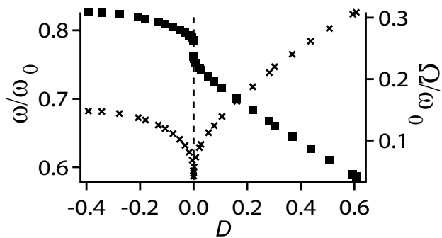
Figure 11: Evolution of the main frequency \omega (squares) and the beating \Omega (crosses) for different trajectories, for \alpha = 0.5 and E = -1.02 . Trajectories are identified through the point where they intersect a line linking the quadrature and the antiphase solution. D is the distance between the intersection point and the separatrix. The quadrature (resp. antiphase) solution is in D = -0.4 (resp. D = 0.6 ).
