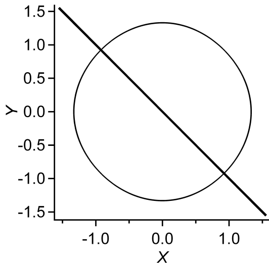
Figure 6: Real space trajectories for the antiphase and the quadrature solutions, calculated for \alpha = 0.5 , E = -1.02 . The antiphase solution consists in an oscillation of the atom along the straight line, while the quadrature solutions correspond to a rotation of the atom along the circle.
