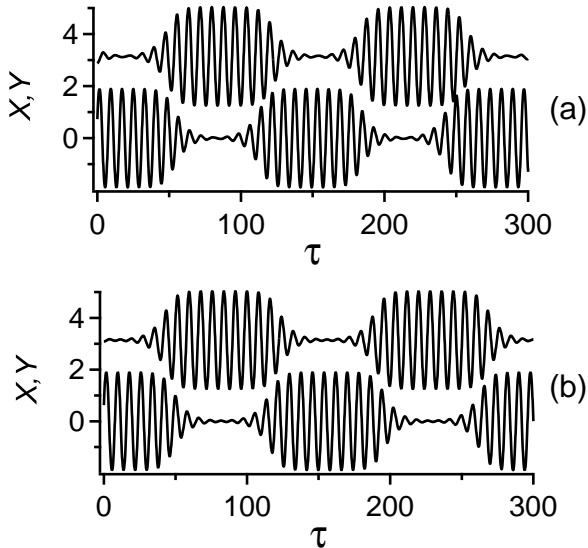
Figure 9: Motion of the atoms as a function of the time \tau = \omega_0 t , for \alpha = 0.5 and E = -1.02 , for initial conditions close to the unstable periodic orbits. In both plots, X and Y trajectories are centered on 0, but for sake of clarity, the Y trajectories have been shifted by \pi , so that they appear to be centered on \pi . The corresponding trajectories are on tori centered on (a) the antiphase periodic orbit and (b) a quadrature periodic orbit.
