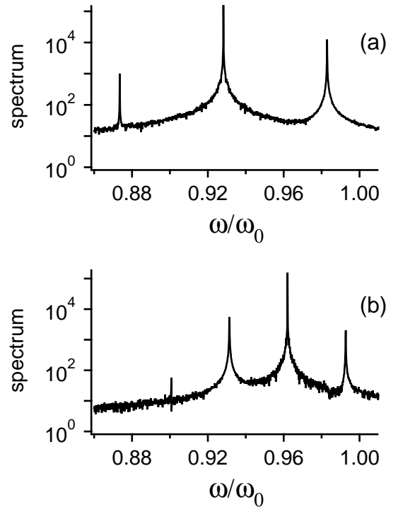
Figure 4: Spectrum of the atomic motion along the X direction, in the vicinity of the (a) anti-phase solution, and (b) quadrature solution. These are respectively the FFT of the signals of Figs 3b and 3c. Both spectra are represented with the same scales, to make the comparison easier.
