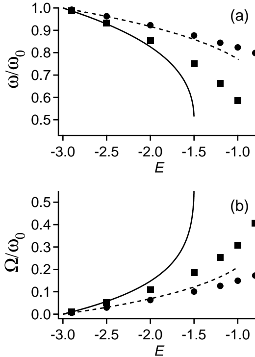
Figure 7: Oscillation frequencies of the atom in the vicinity of the periodic orbits. In (a), frequency of the periodic solution; in (b), frequency of the beating. The solid (resp. dotted) lines are the same as in Fig. 2, i.e. they refer to the analytical in phase (resp. in quadrature) frequencies in the Duffing approximation. The square (resp. round) markers refer to the values computed, through numerical simulations of the full model, for the in-phase (resp. in-quadrature) solutions.
