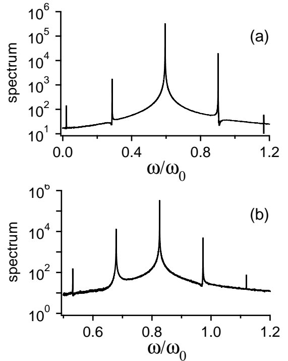
Figure 8: Spectrum of the atomic motion along the X direction, in the vicinity of the (a) antiphase solution, and (b) quadrature solution for \alpha = 0.5 , E = -1.02 . The corresponding trajectories give the Poincaré sections which are the first circles around the periodic solutions in Fig. 5. In (a), Poincaré section crossing the \dot{X} = 0 axis in X = 1.46 . In (b), Poincaré section crossing the X = 0 axis in \dot{X} = 1.195 .
