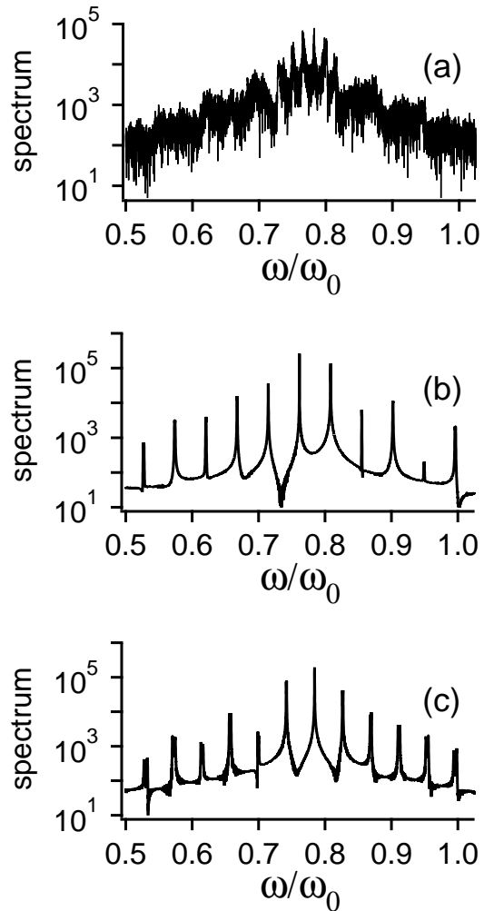
Figure 10: Spectrum of atomic trajectories close to the unstable periodic cycles, in (a) the chaotic area, (b) on the side of the antiphase solution and (c) on the side of a quadrature solution.
