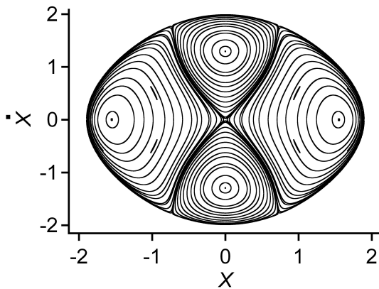
Figure 5: Poincaré sections for \alpha = 0.5 and E = -1.02 .
