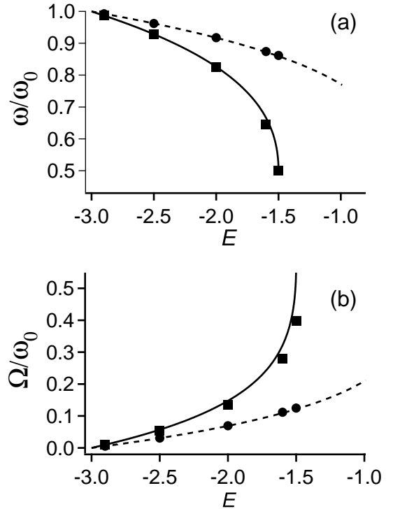
Figure 2: Oscillation frequencies of the atom in the vicinity of the periodic orbits, in the case of the Duffing approximation. In (a), frequency of the periodic solution; in (b), frequency of the analytical in-phase (resp. quadrature) frequencies. The square (resp. round) markers refer to the values computed through numerical simulations, of the in-phase (resp. quadrature) solutions.
