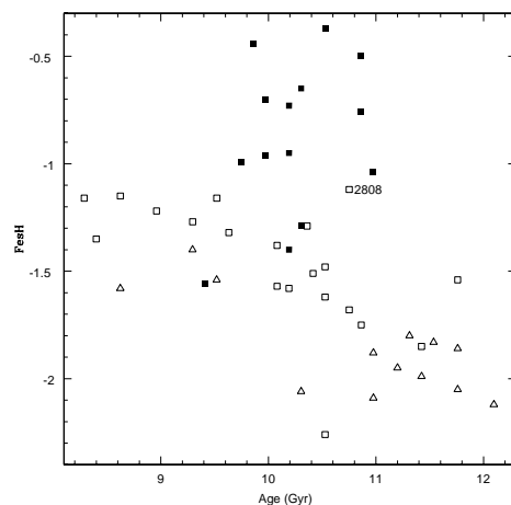
Figure 3. Age-metallicity diagram. Same symbols as Fig. 2. No age estimate is available for NGC 6139, 6229, 6304, 6388, 6441, 6569 and 6642. Metallicity decreases with age in the halo clusters while it very marginally increases with age in the disc clusters
